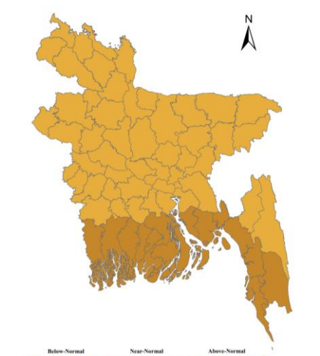
Probabilistic Multi-Model Ensemble Rainfall Forecast for ASO
